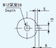
附带键轴 Shaft with key
